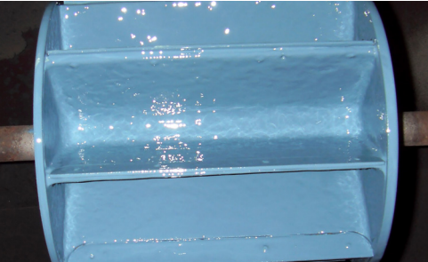
Belzona 1321 (Ceramic S-Metal) Ceramic-filled, erosion-corrosion-resistant epoxy coating. Approved for contact with drinking water (e.g. WRAS).
