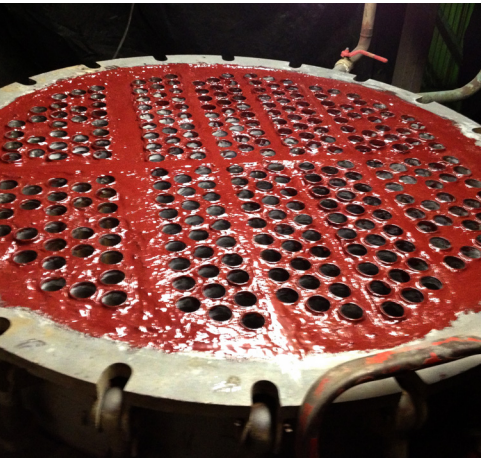
Belzona 4341 (Magma CR4) Epoxy novolac barrier coating for concrete and metal protection, offering high resistance to hot inorganic acids.
