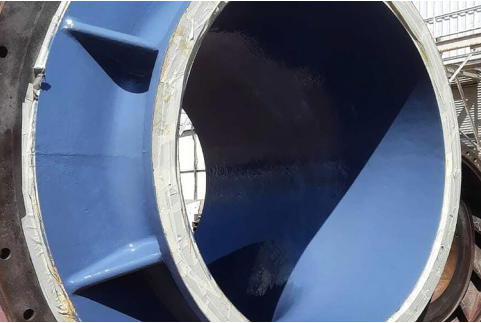
Belzona 5821 Ceramic-filled epoxy coating for erosion, corrosion and chemical protection of high erosion fluid flow areas.
