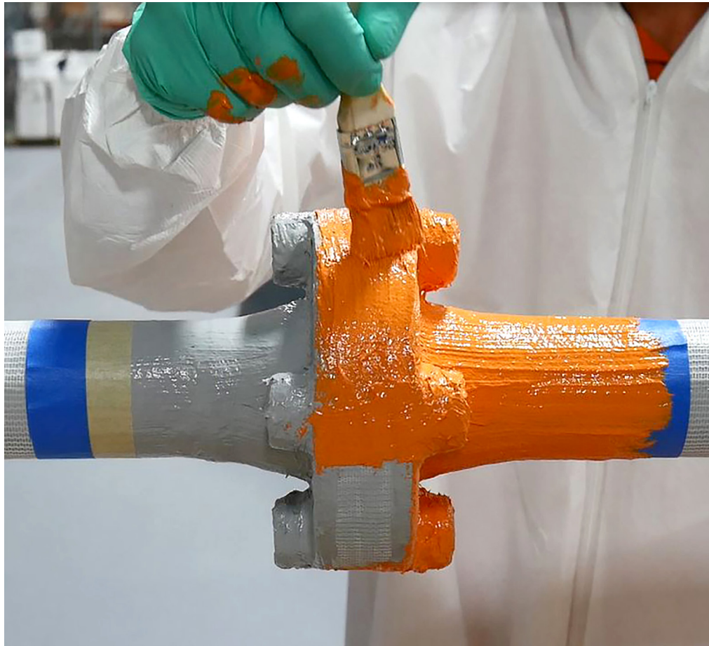
Belzona 3412 Peelable, hybrid elastomeric encapsulating system for the protection of flanges and pipework against crevice, galvanic and atmospheric corrosion.
