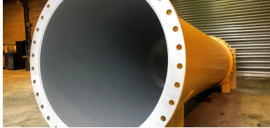
Belzona 5811 Epoxy coating for corrosion and chemical protection under immersion in aqueous solutions at temperatures up to 50°C (122°F).
