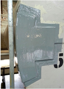
Belzona 1212 High-performance, rapid-curing, surface-tolerant epoxy repair composite suitable for wet and oily surfaces. Approved for contact with drinking water (e.g. WRAS).
